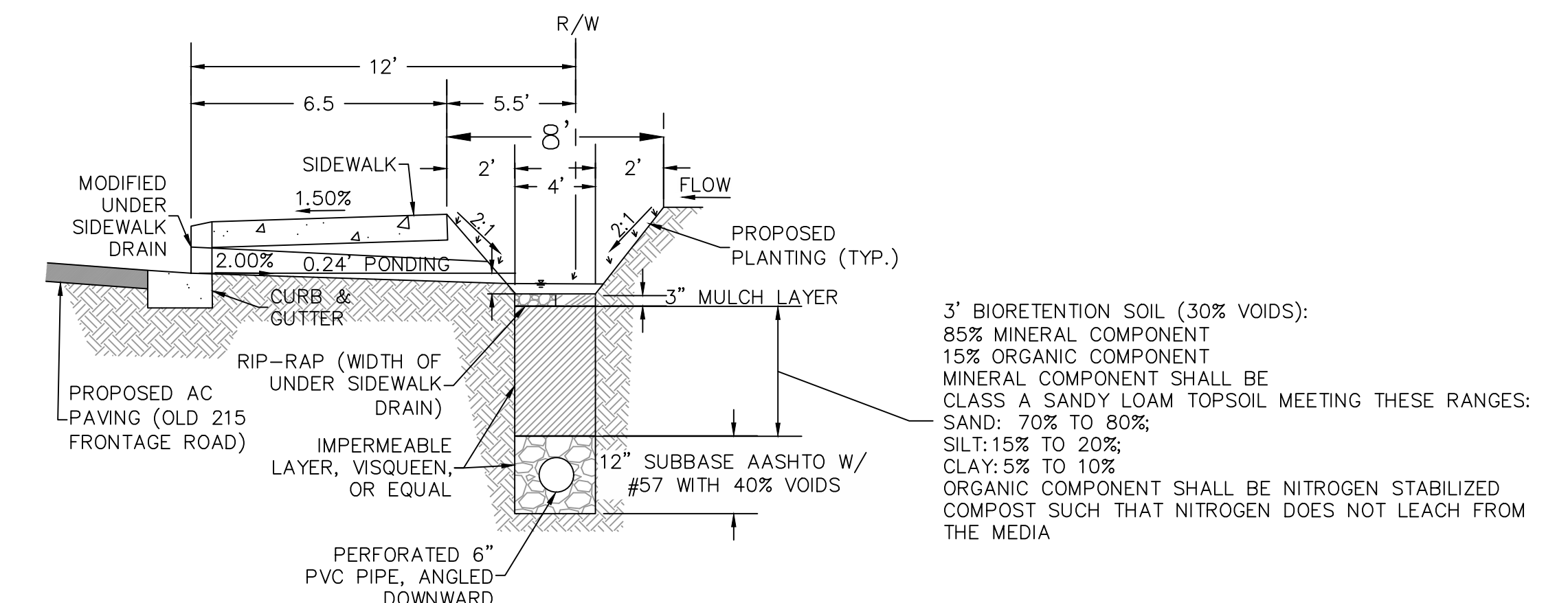
BIOSWALE DETAIL FOR OLD 215 FRONTAGE ROAD
