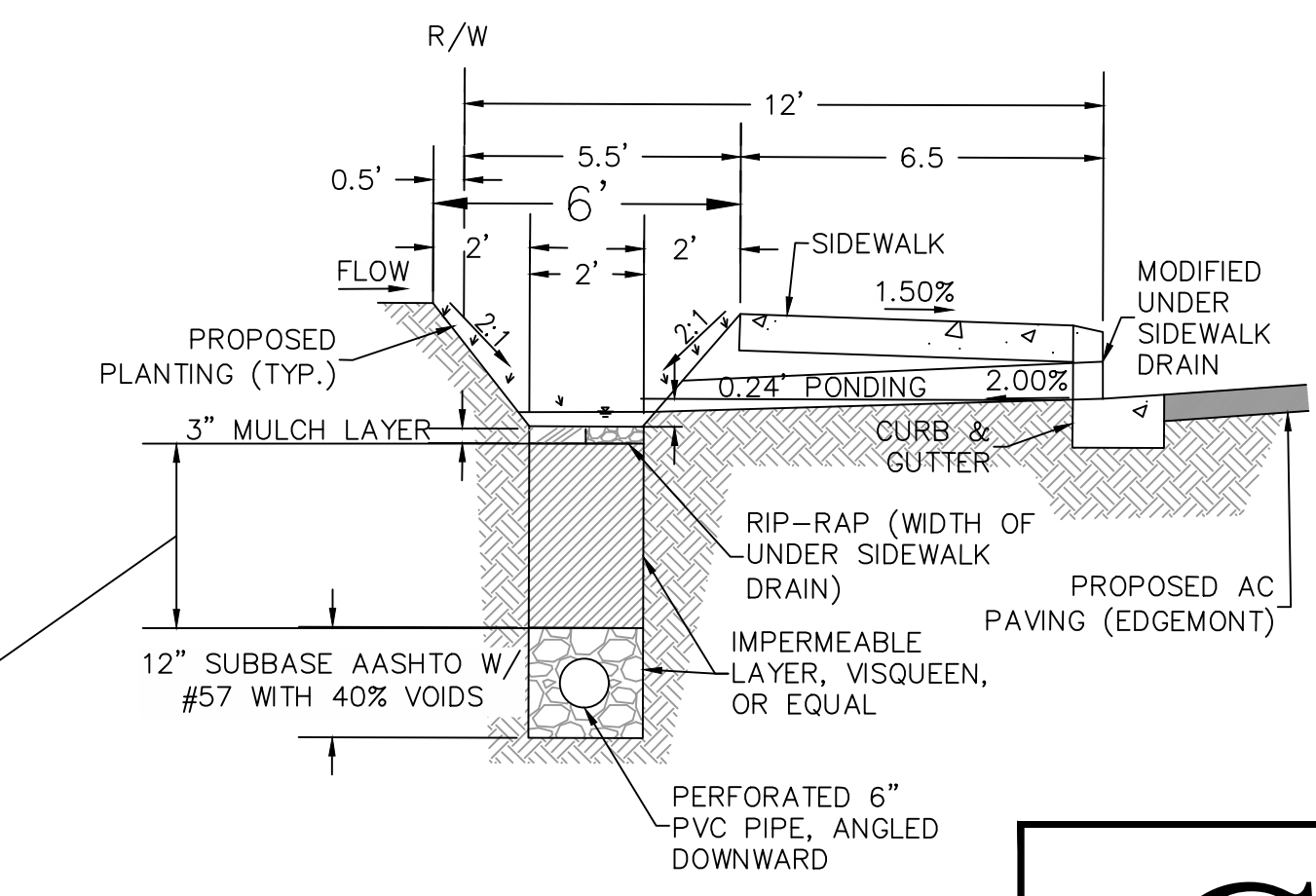
BIOSWALE DETAIL FOR EDMONT STREET
